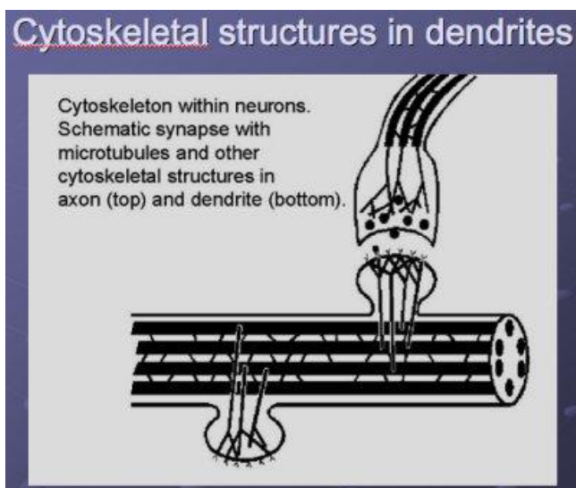
Image 2: Cytoskeletal Structures in Dendrites
