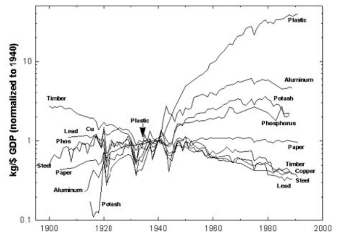
Image 1: U.S. Materials Intensity of Use
