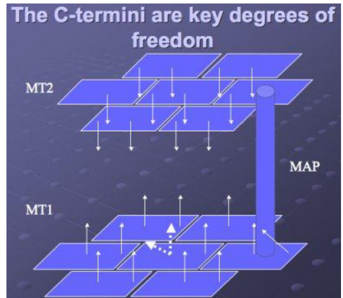
Image 4: MAPs Connecting Microtubules
