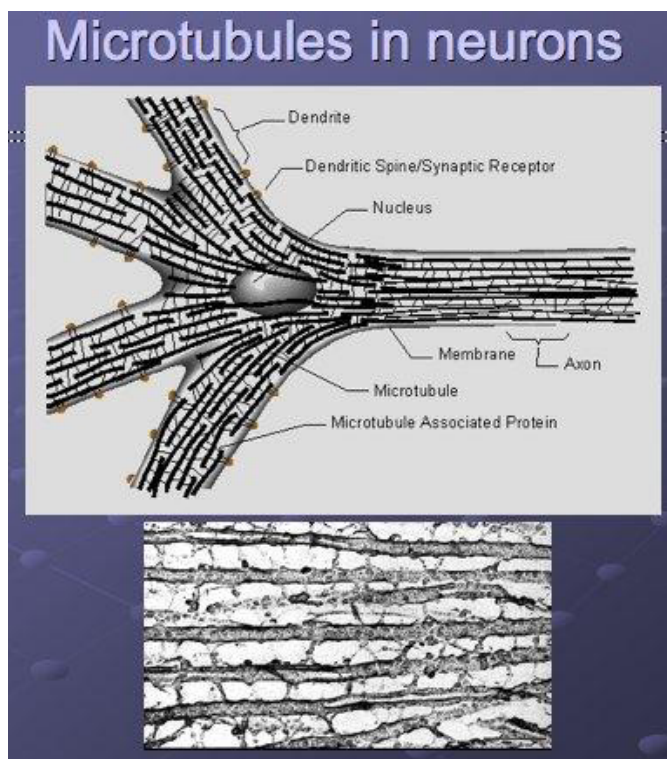
Image 1: Microtubules in Neurons
